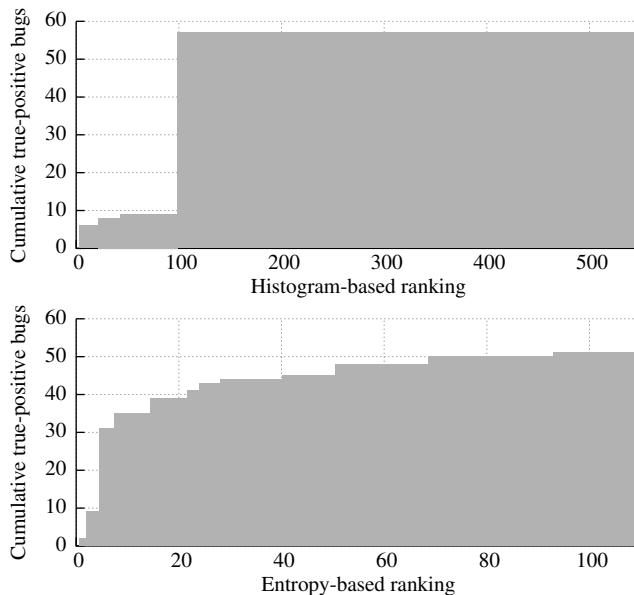
Figure 7: Cumulative true-positive bugs, sorted by ranking reported by JUXTA. For histogram-based checkers, bug reports are ranked in descending order, while for entropy-based checkers, bug reports (except for ones with zero entropy) are ranked in ascending order. JUXTA’s statistical path comparison and bug report ranking can effectively save programmers effort by letting them investigate the highest-ranked reports first.
