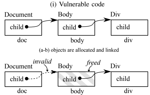
(ii) Objects and their relations in the course of running (i)
